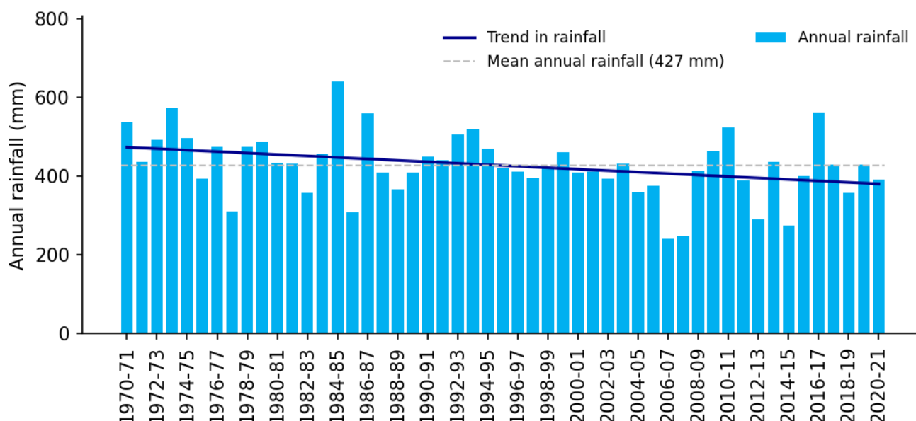
Figure 3.10 Annual rainfall for 1970–71 to 2020–21 at the Tintinara rainfall station (BoM station 25514)
