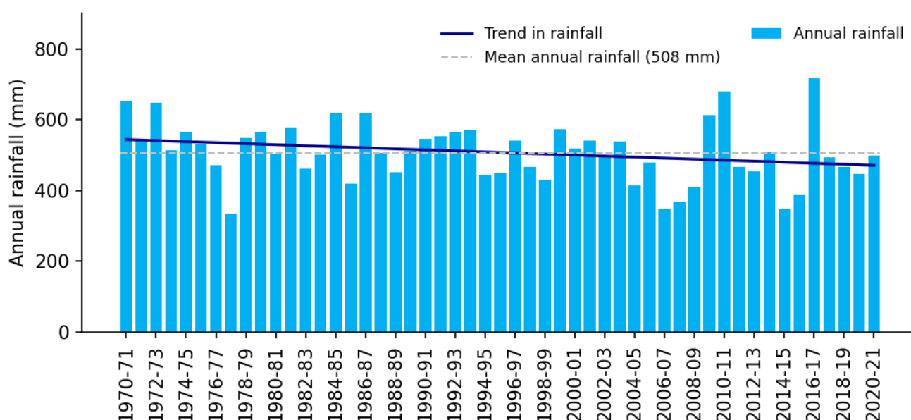
Figure 3.6 Annual rainfall for 1970–71 to 2020–21 at the Marcollat rainfall station (BoM station 26017)
