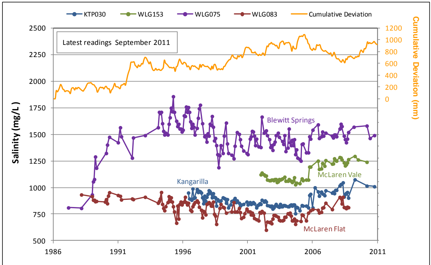
Figure 19. Groundwater salinity trends for the Maslin Sands Aquifer in the McLaren Vale PWA
