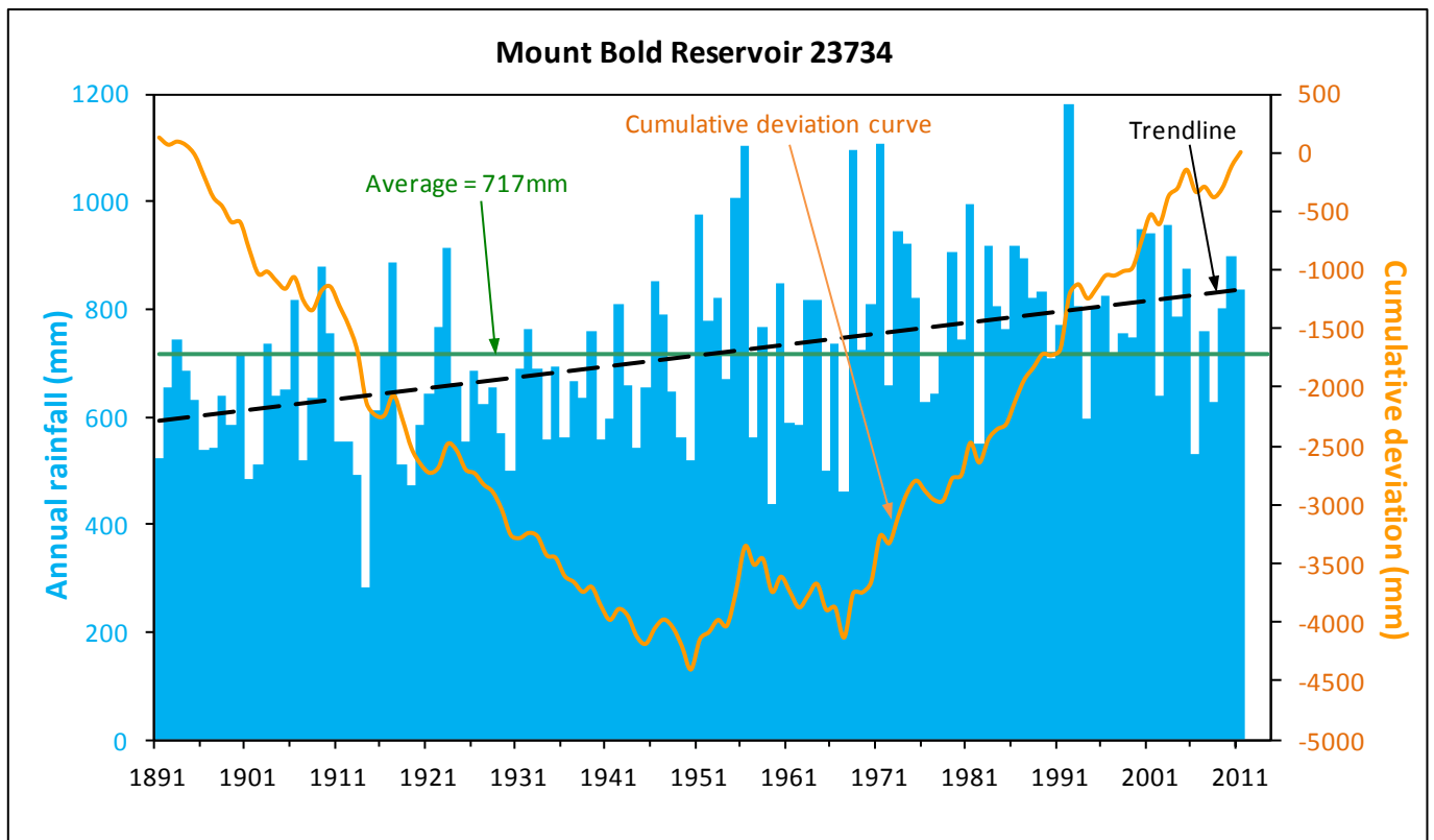
Figure 7. Annual rainfall and cumulative deviation from mean annual rainfall at Mount Bold in the McLaren Vale PWA
