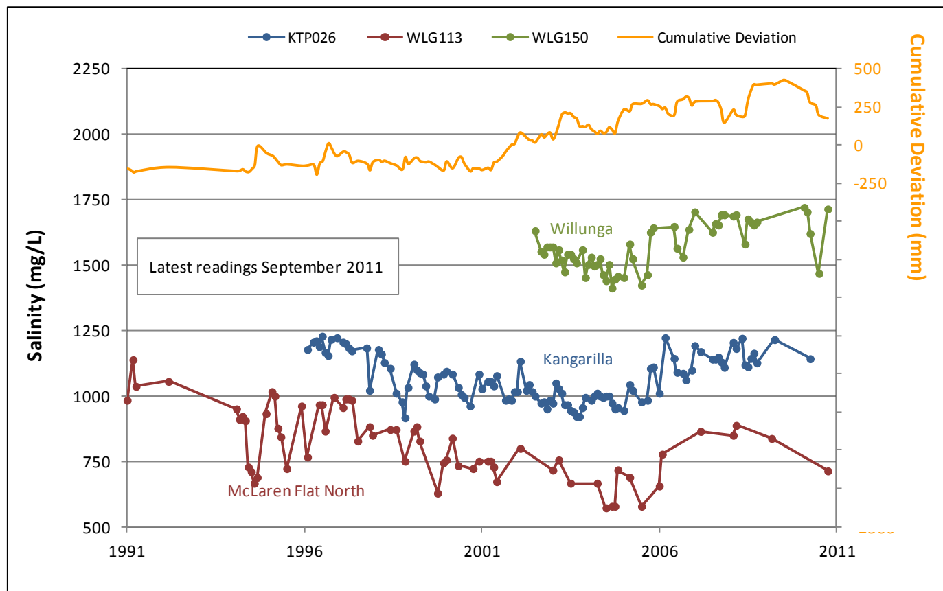
Figure 18. Groundwater salinity trends for the Port Willunga Formation Aquifer in the McLaren Vale PWA
