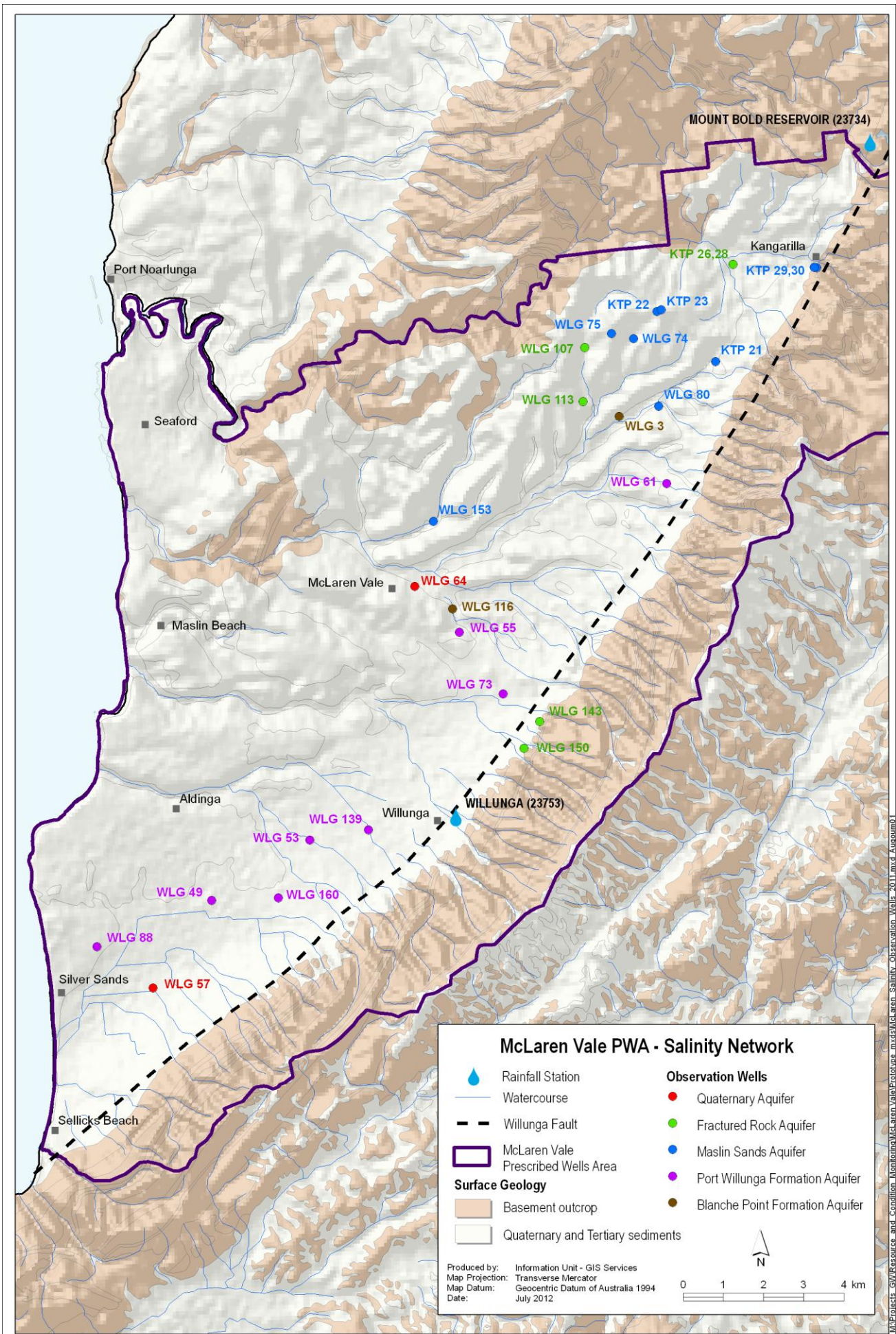
Figure 12. Location of groundwater salinity observation wells in the McLaren Vale PWA
