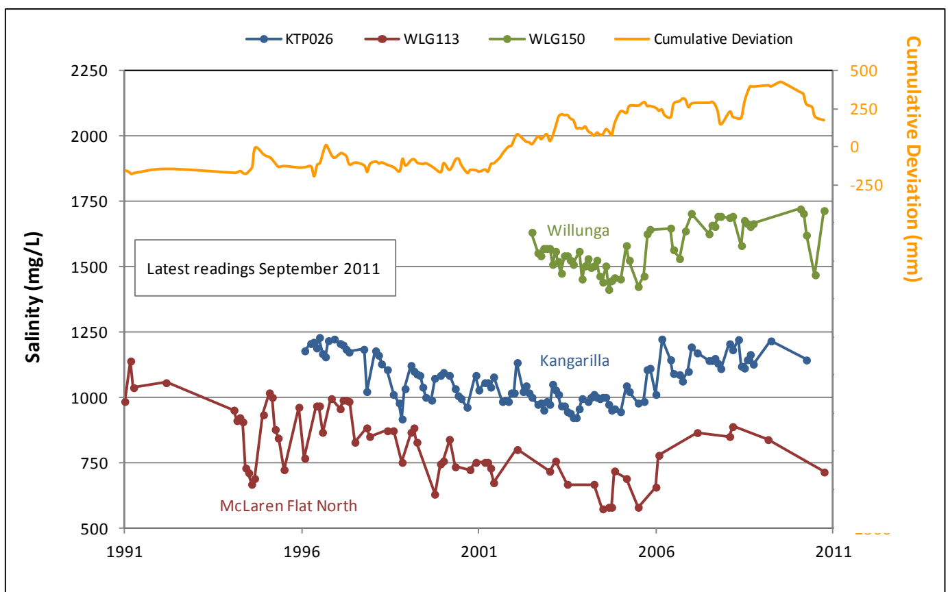
Figure 20. Groundwater salinity trends of the Fractured Rock Aquifer in the McLaren Vale PWA
