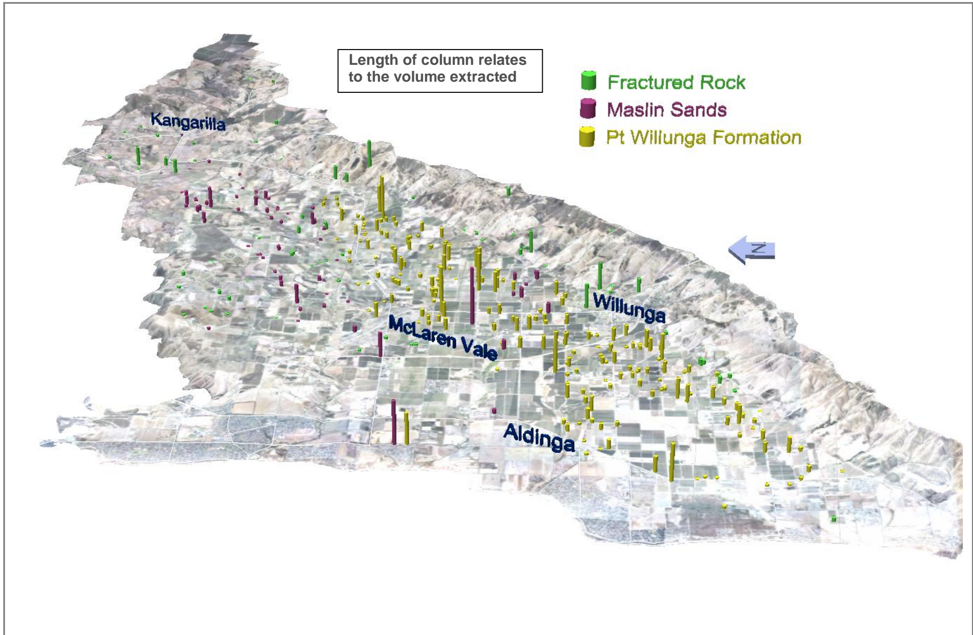
Figure 10. Spatial distribution of licensed groundwater extraction from each well during the 2010–11 irrigation season in the McLaren Vale PWA
