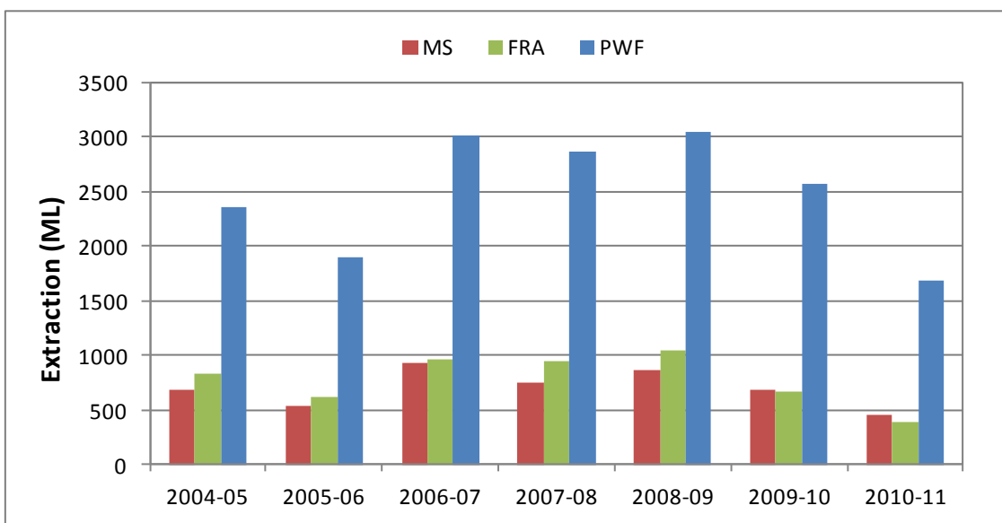
Figure 9. Historic licensed groundwater use by aquifer type for the McLaren Vale PWA
