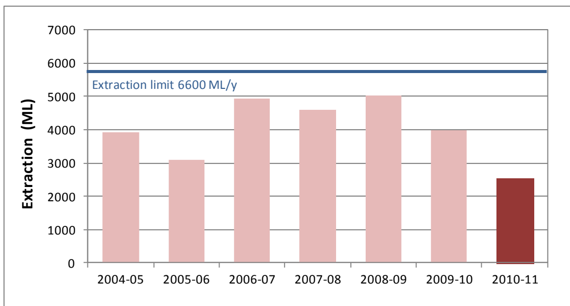
Figure 8. Historic licensed groundwater use in the McLaren Vale PWA
