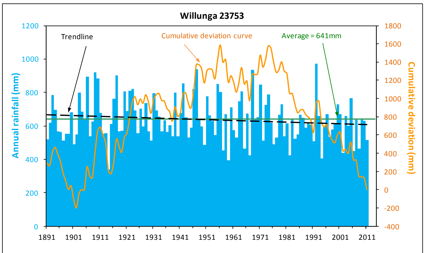
Figure 6. Annual rainfall and cumulative deviation from mean annual rainfall at Willunga in the McLaren Vale PWA
