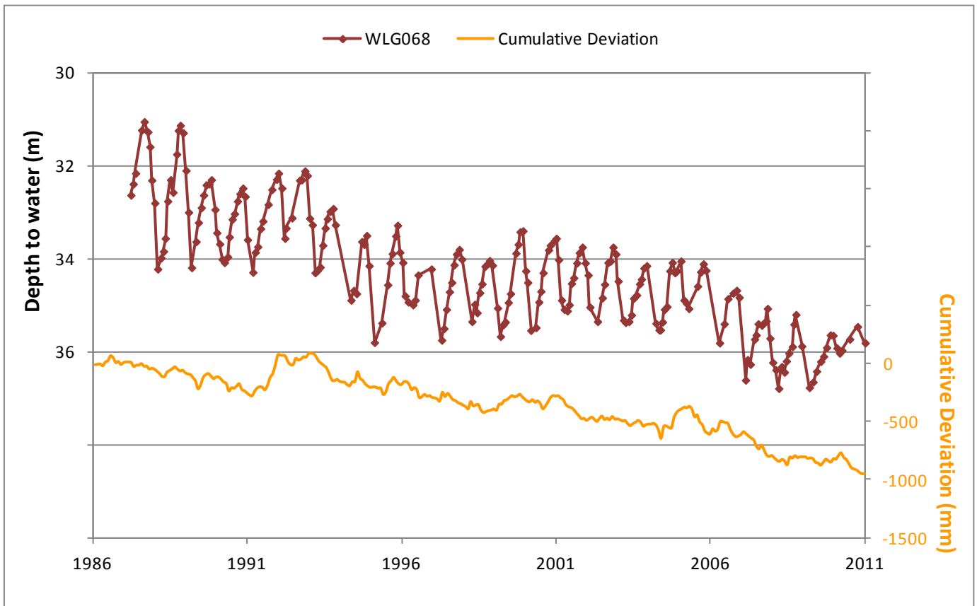
Figure 14. Comparison of rainfall monthly cumulative deviation and groundwater level trends of the PWA Aquifer in the McLaren Vale PWA
