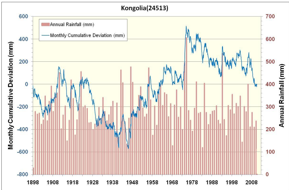
Figure 7. Annual rainfall and cumulative deviation from mean monthly rainfall for Kongolia station in the Marne–Saunders PWRA
