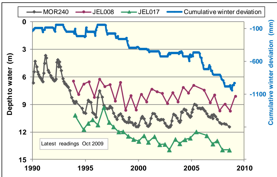
Figure 17. Groundwater level trends of the fractured rock aquifer in the Marne–Saunders PWRA
