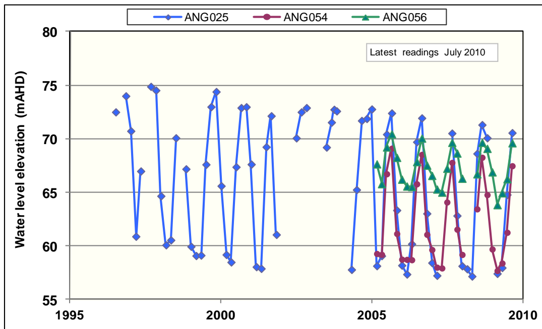
Figure 15. Groundwater level trends of the confined limestone aquifer in the Marne-Saunders PWRA
