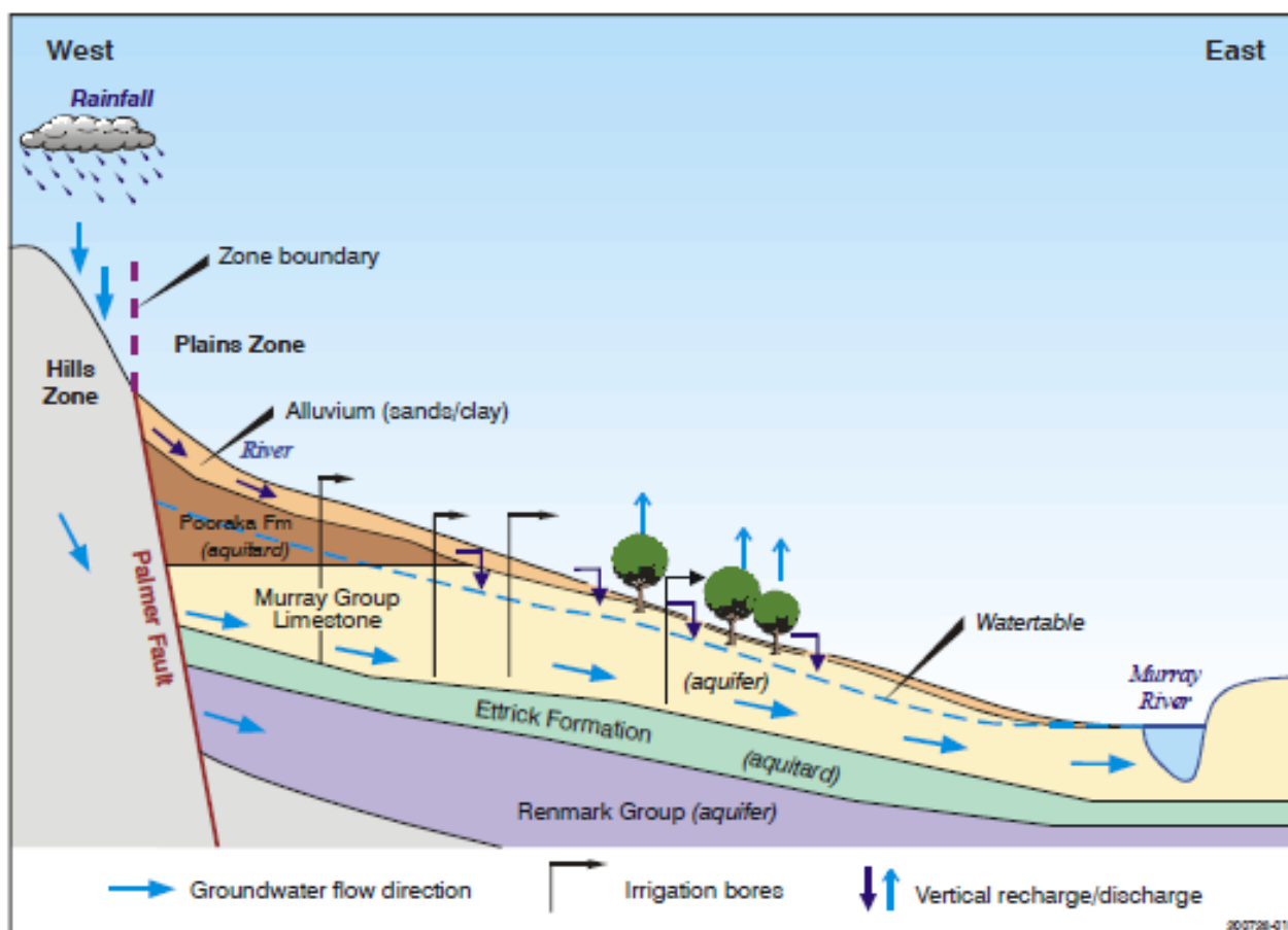
Figure 2. Schematic cross section of the Marne–Saunders PWRA
