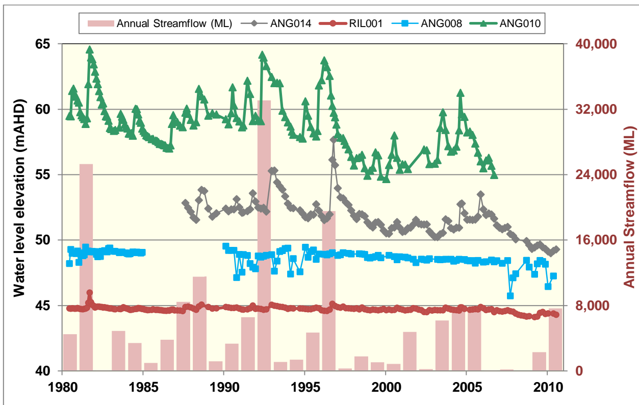
Figure 16. Groundwater level trends of the unconfined limestone aquifer in the Marne–Saunders PWRA
