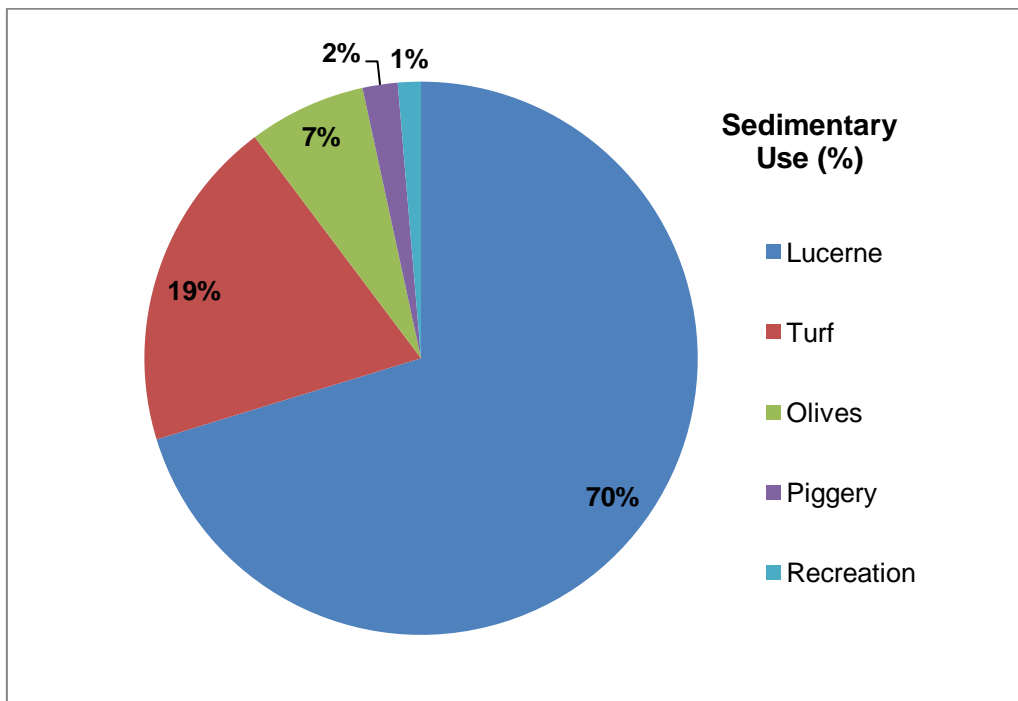
Figure 10. Groundwater proportions extracted per type of use in the sedimentary aquifer of the Marne–Saunders PWRA for 2009/10
