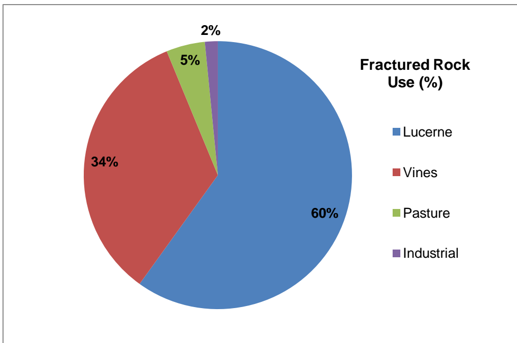
Figure 9. Groundwater proportions extracted per type of use in the fractured rock aquifer of the Marne–Saunders PWRA for 2009/10
