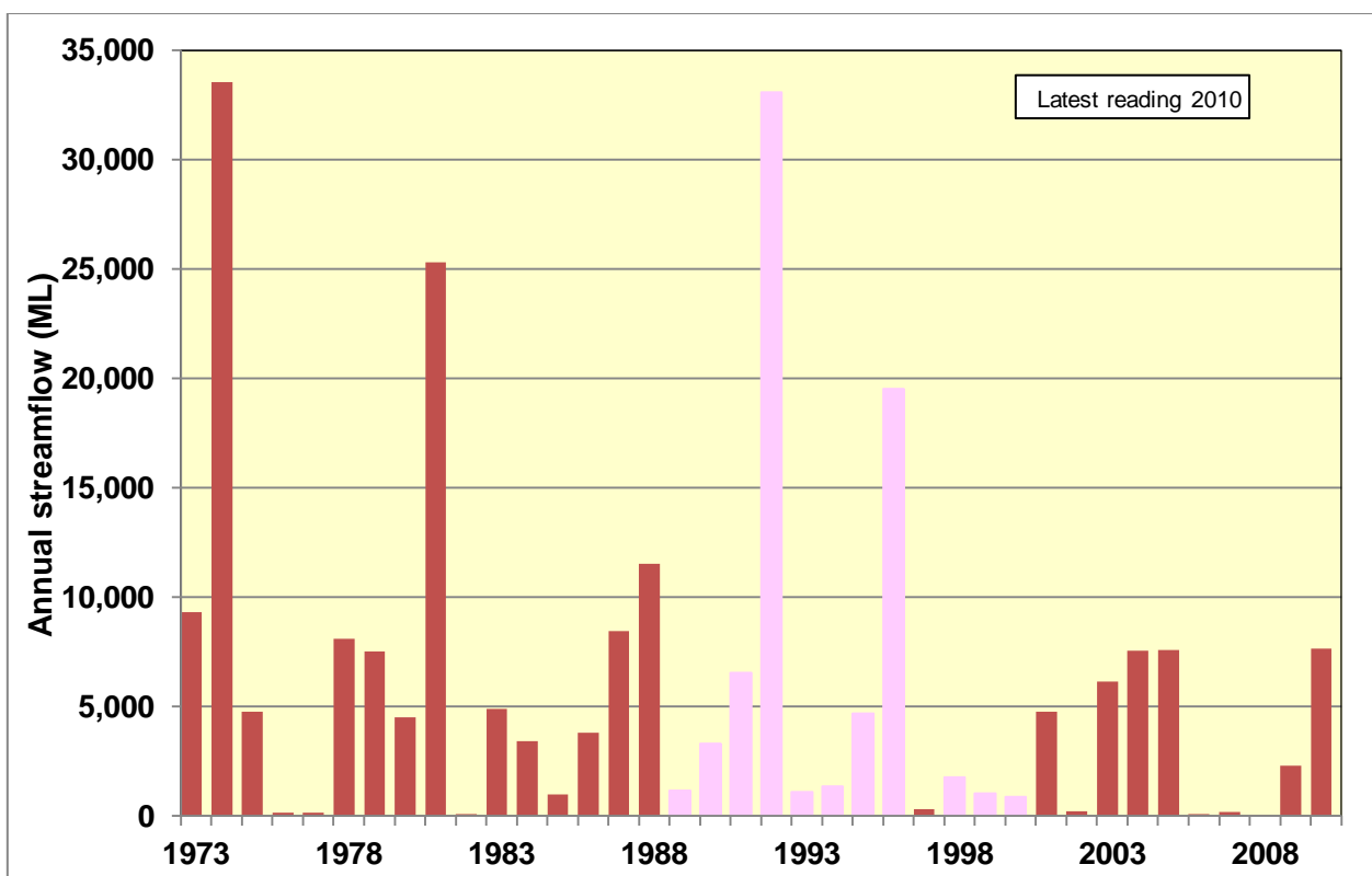
Figure 13. Annual streamflow at the Marne Gorge flow gauging station in the Marne-Saunders PWRA
