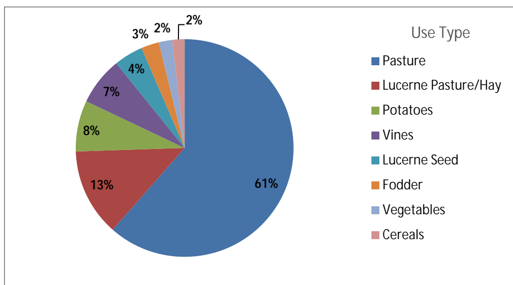
Figure 12. Groundwater proportions used per type of crop for the Lower Limestone Coast PWA in 2008–09
