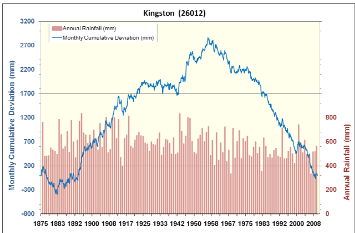
Figure 9. Annual rainfall and monthly cumulative deviation for Kingston in the Lower Limestone Coast PWA
