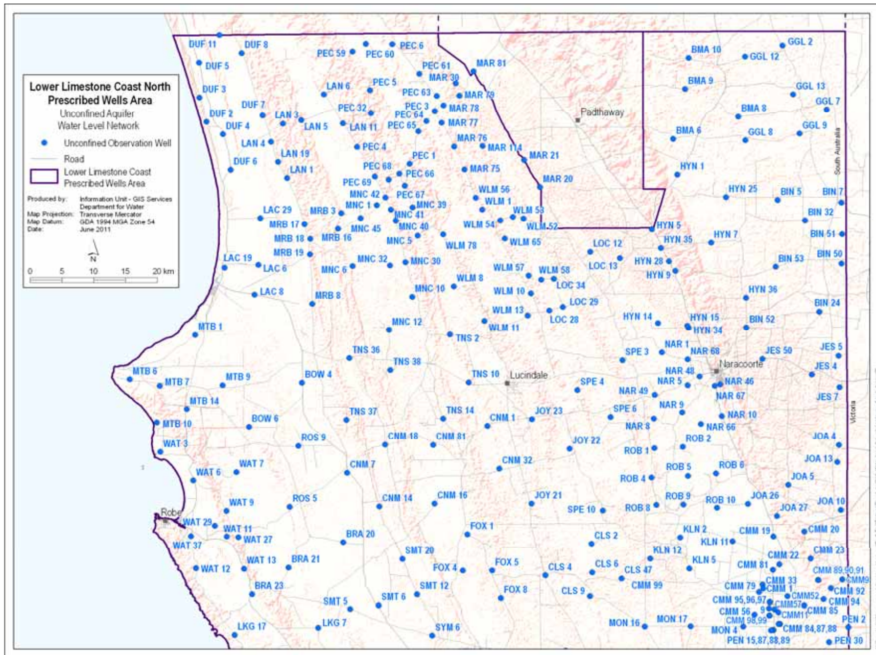
Figure 13. Location of water level observation wells for the unconfined aquifer in the northern part of the Lower Limestone Coast PWA
