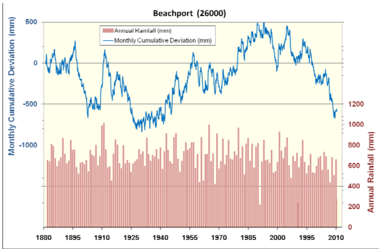
Figure 8. Annual rainfall and monthly cumulative deviation for Beachport in the Lower Limestone Coast PWA
