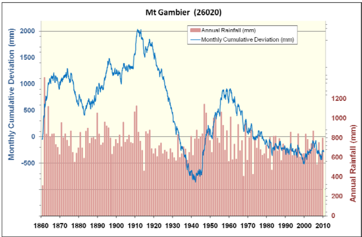
Figure 6. Annual rainfall and monthly cumulative deviation for Mount Gambier in the Lower Limestone Coast PWA
